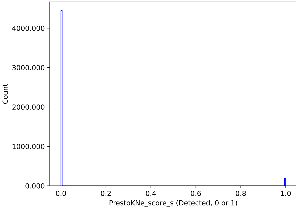
too_elab_r32_d2_giz_v3.4_10yrs : PrestoKNe_score_s
