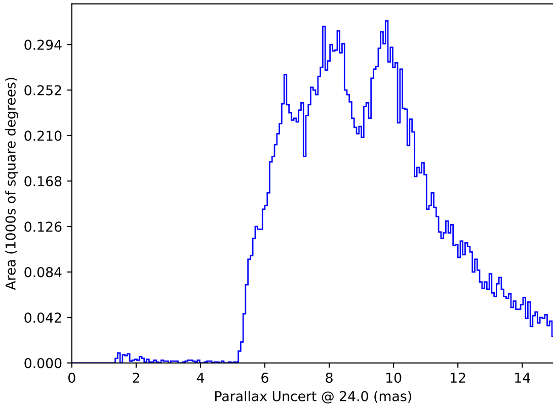
too_elab_r32_d2_giz_v3.4_10yrs : Parallax Uncert @ 24.0
