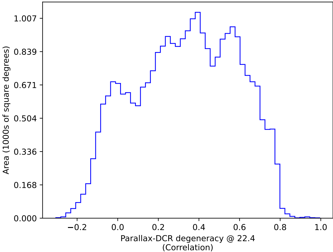
too_elab_r32_d2_giz_v3.4_10yrs : Parallax-DCR degeneracy @ 22.4
