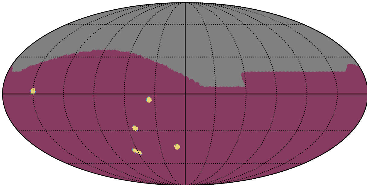
too_elab_r32_d2_giz_v3.4_10yrs : NumberOfQuickRevisits
