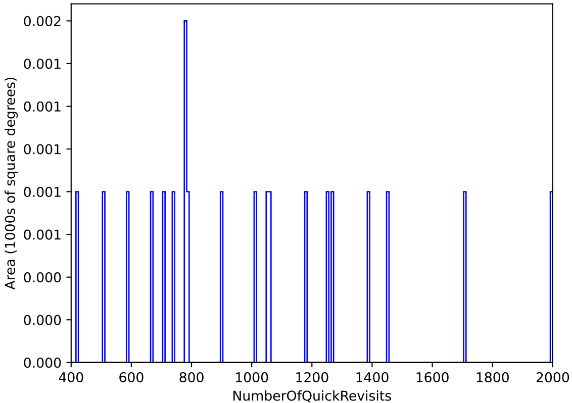
too_elab_r32_d2_giz_v3.4_10yrs : NumberOfQuickRevisits
