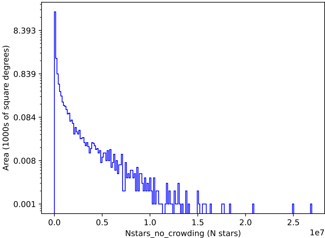
too_elab_r32_d2_giz_v3.4_10yrs z: Nstars_no_crowding
