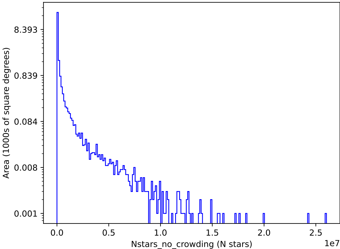
too_elab_r32_d2_giz_v3.4_10yrs y: Nstars_no_crowding
