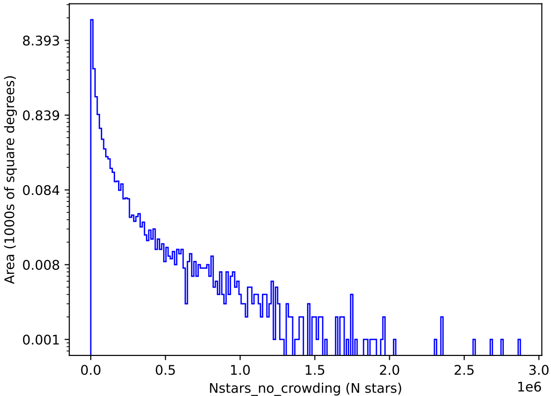
too_elab_r32_d2_giz_v3.4_10yrs u: Nstars_no_crowding
