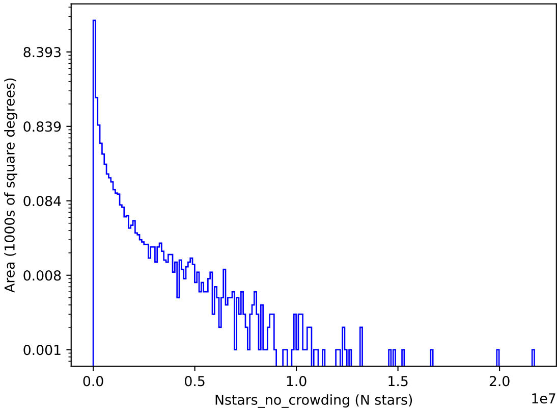
too_elab_r32_d2_giz_v3.4_10yrs r: Nstars_no_crowding
