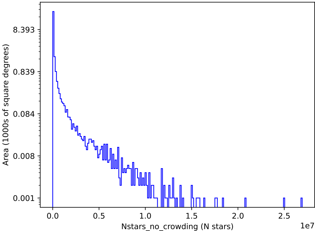
too_elab_r32_d2_giz_v3.4_10yrs i: Nstars_no_crowding
