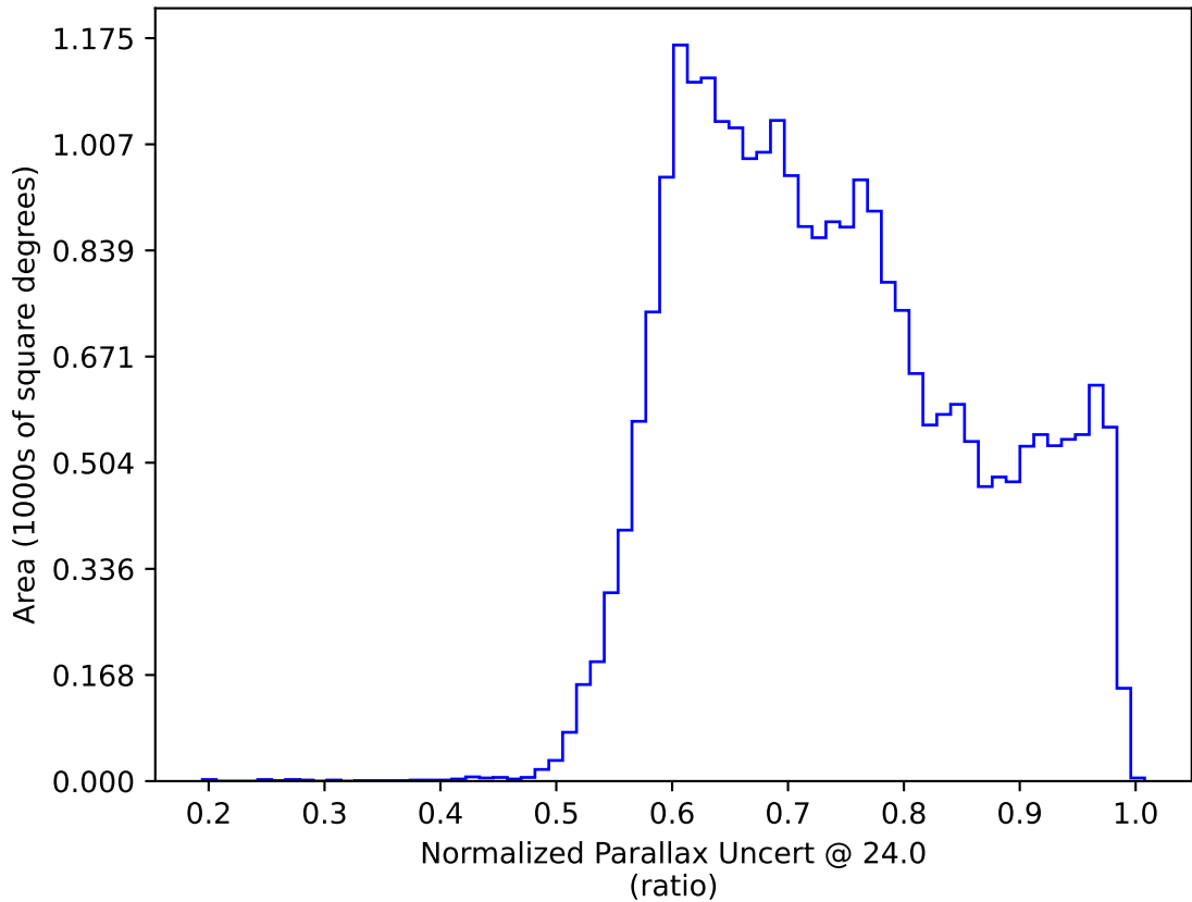
too_elab_r32_d2_giz_v3.4_10yrs : Normalized Parallax Uncert @ 24.0
