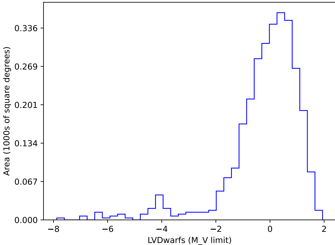
too_elab_r32_d2_giz_v3.4_10yrs gi SCP: LVDwarfs
