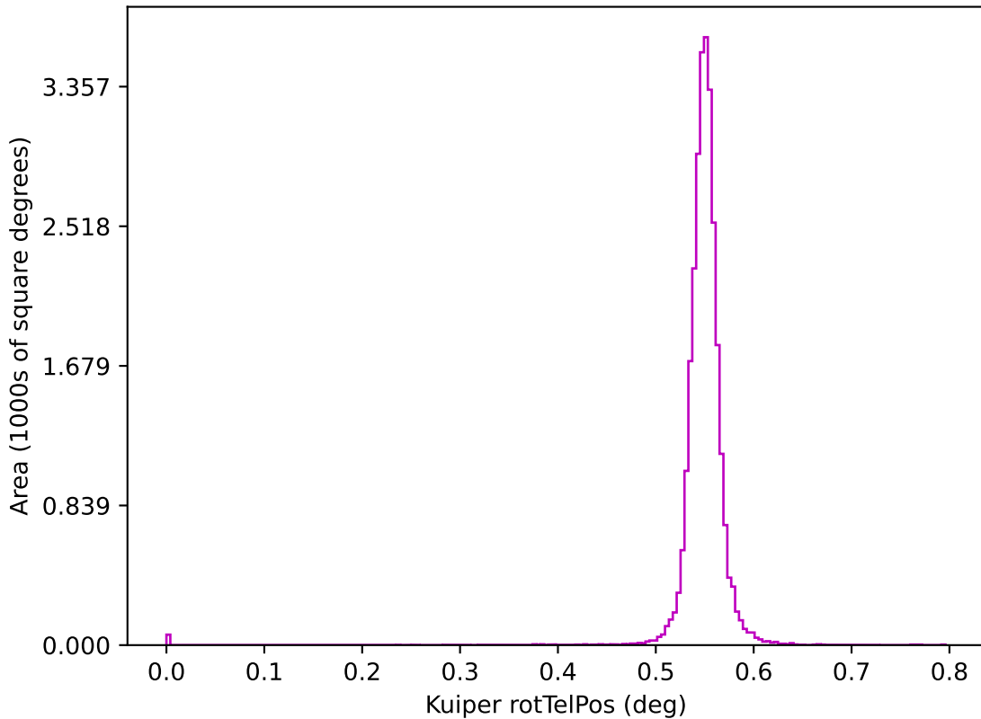
too_elab_r32_d2_giz_v3.4_10yrs z: Kuiper rotTelPos
