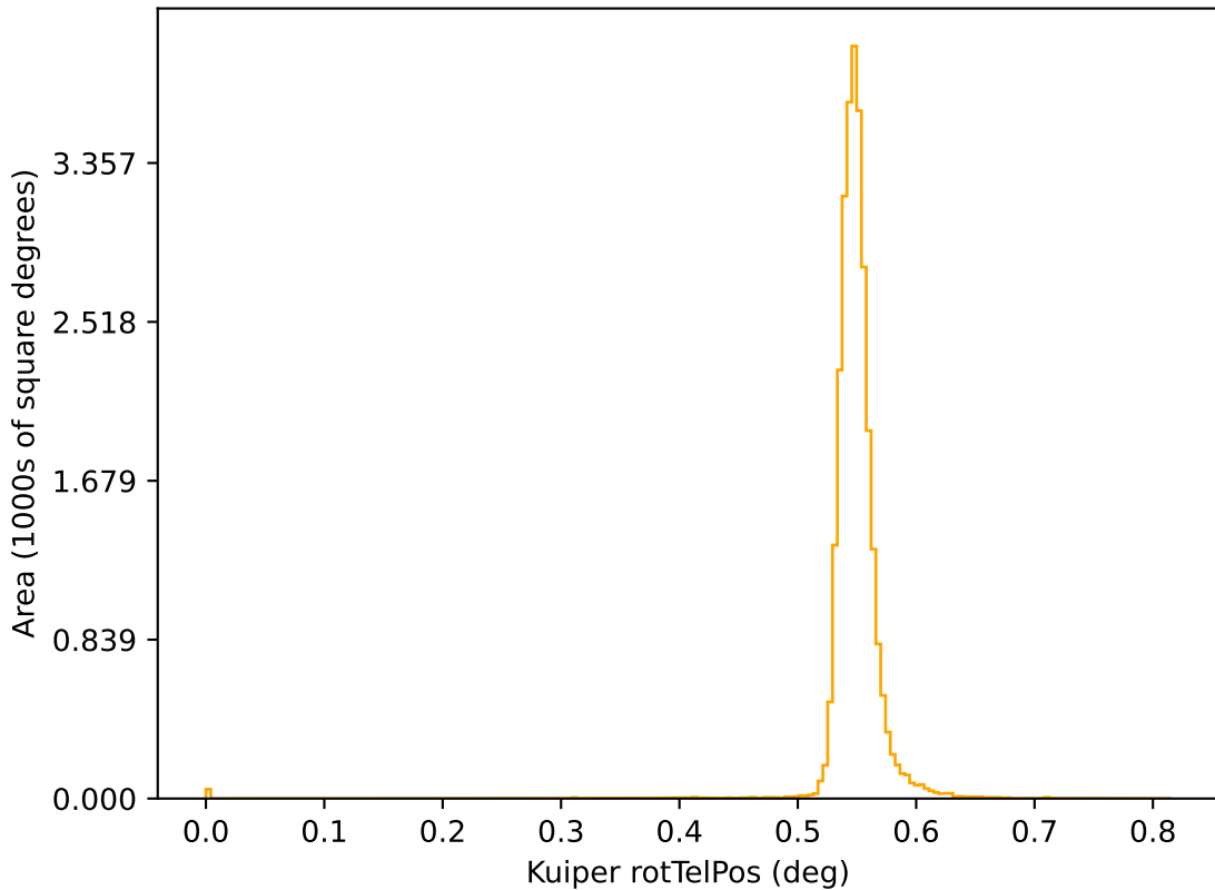
too_elab_r32_d2_giz_v3.4_10yrs r: Kuiper rotTelPos
