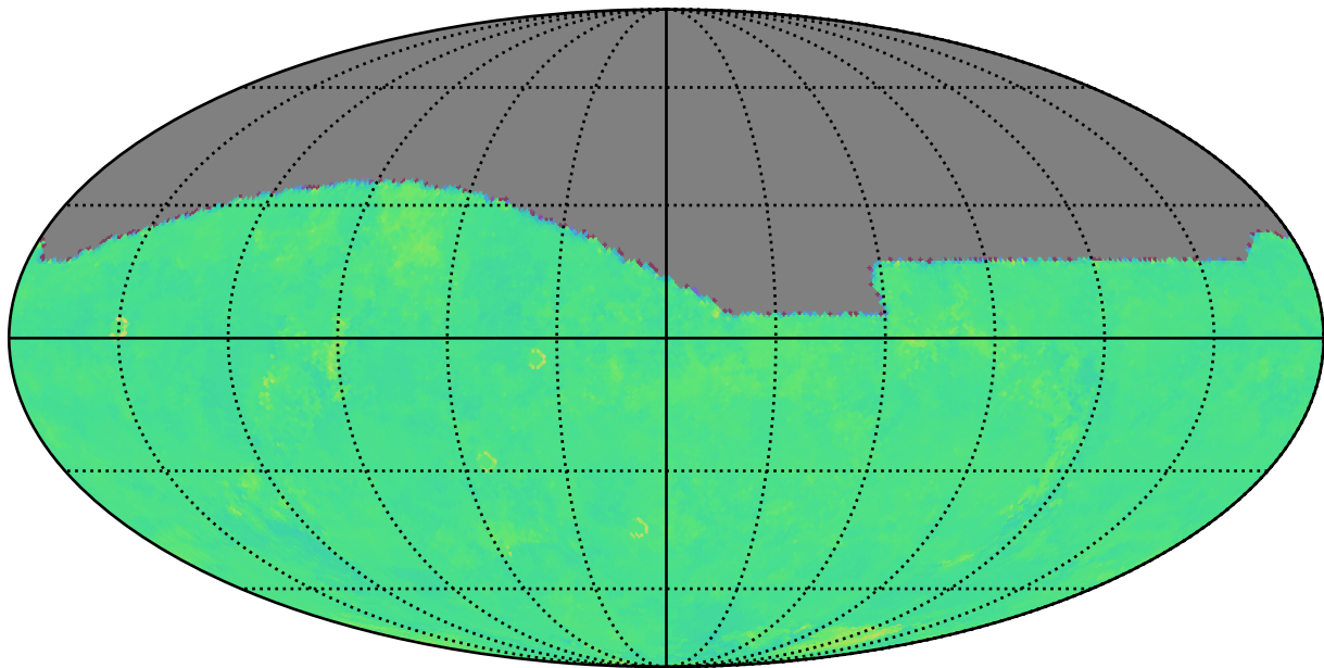
too_elab_r32_d2_giz_v3.4_10yrs g: Kuiper rotTelPos
