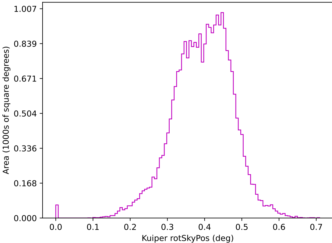
too_elab_r32_d2_giz_v3.4_10yrs z: Kuiper rotSkyPos
