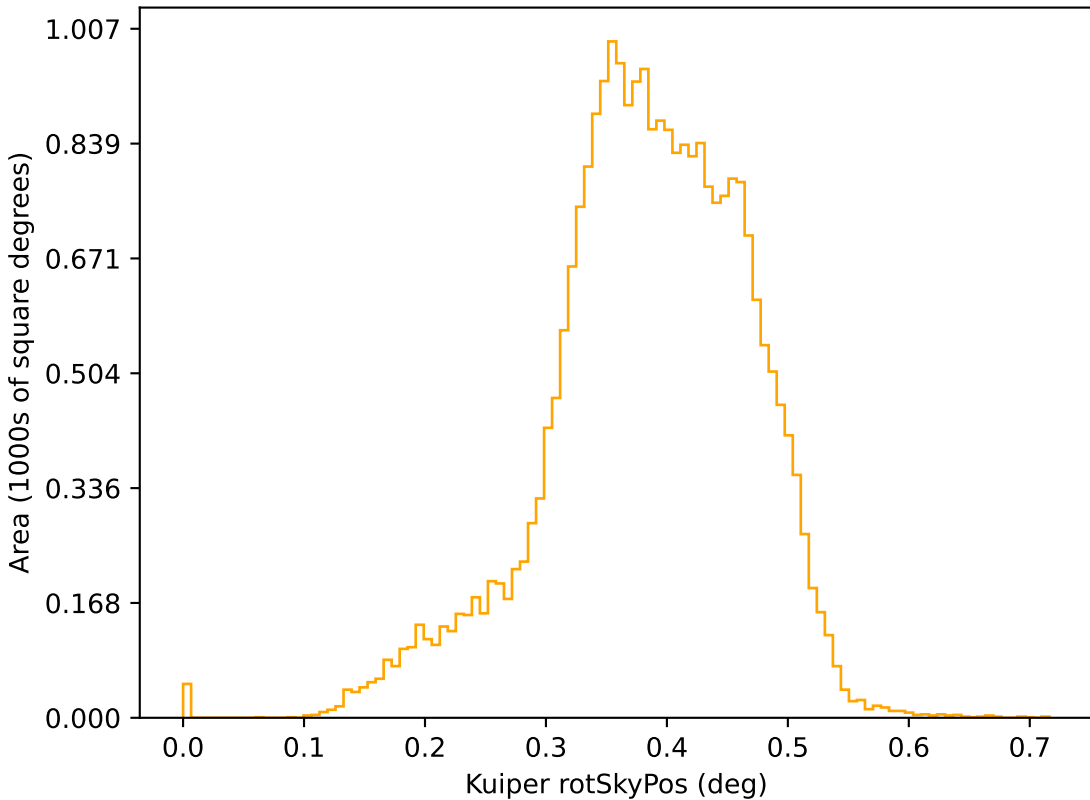
too_elab_r32_d2_giz_v3.4_10yrs r: Kuiper rotSkyPos
