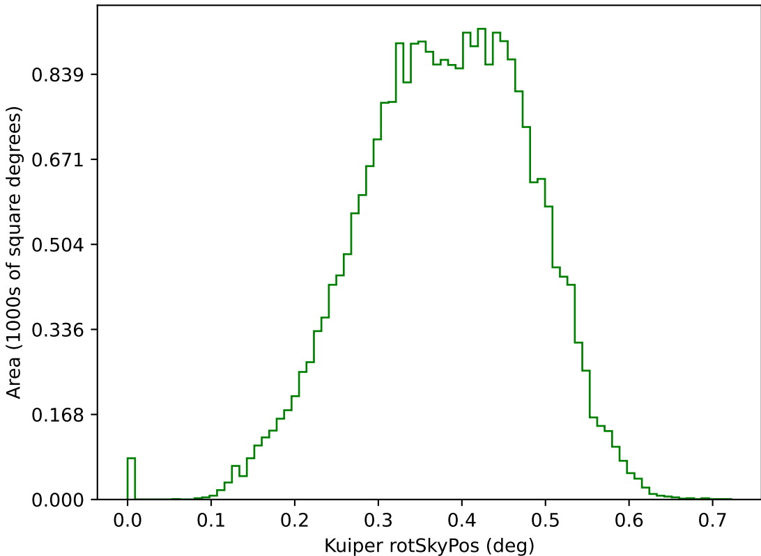
too_elab_r32_d2_giz_v3.4_10yrs g: Kuiper rotSkyPos
