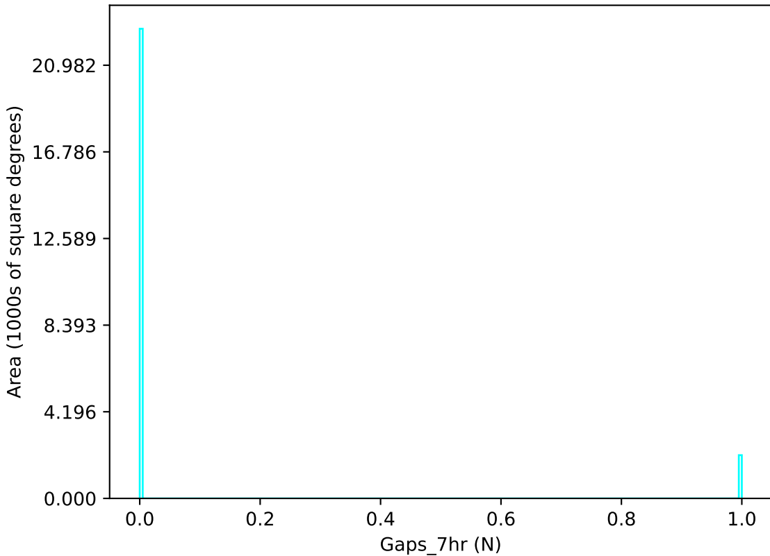
too_elab_r32_d2_giz_v3.4_10yrs u band: Gaps_7hr
