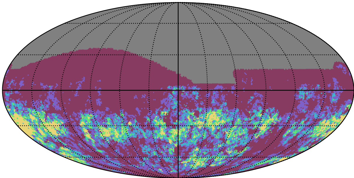
too_elab_r32_d2_giz_v3.4_10yrs r band: Gaps_7hr
