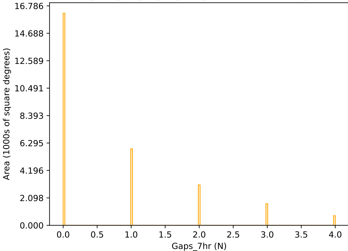
too_elab_r32_d2_giz_v3.4_10yrs r band: Gaps_7hr
