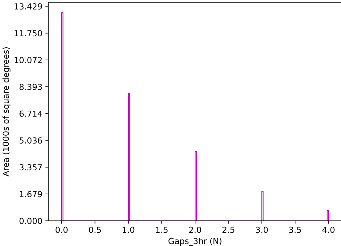
too_elab_r32_d2_giz_v3.4_10yrs z band: Gaps_3hr
