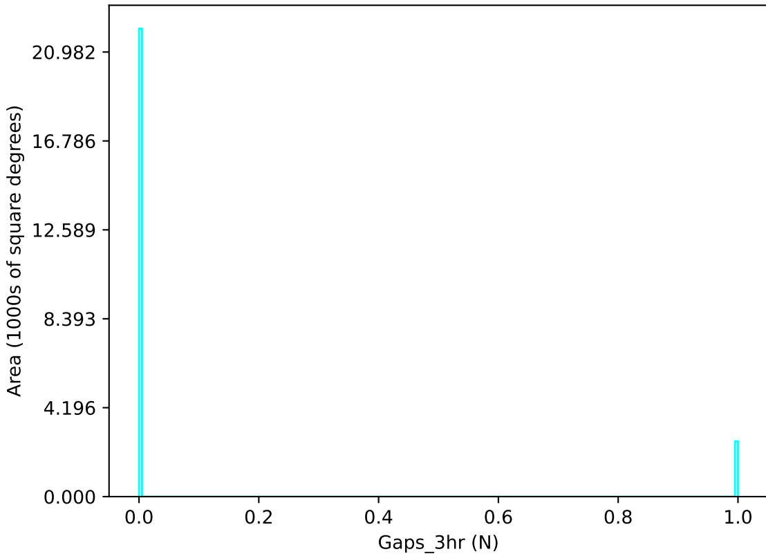
too_elab_r32_d2_giz_v3.4_10yrs u band: Gaps_3hr
