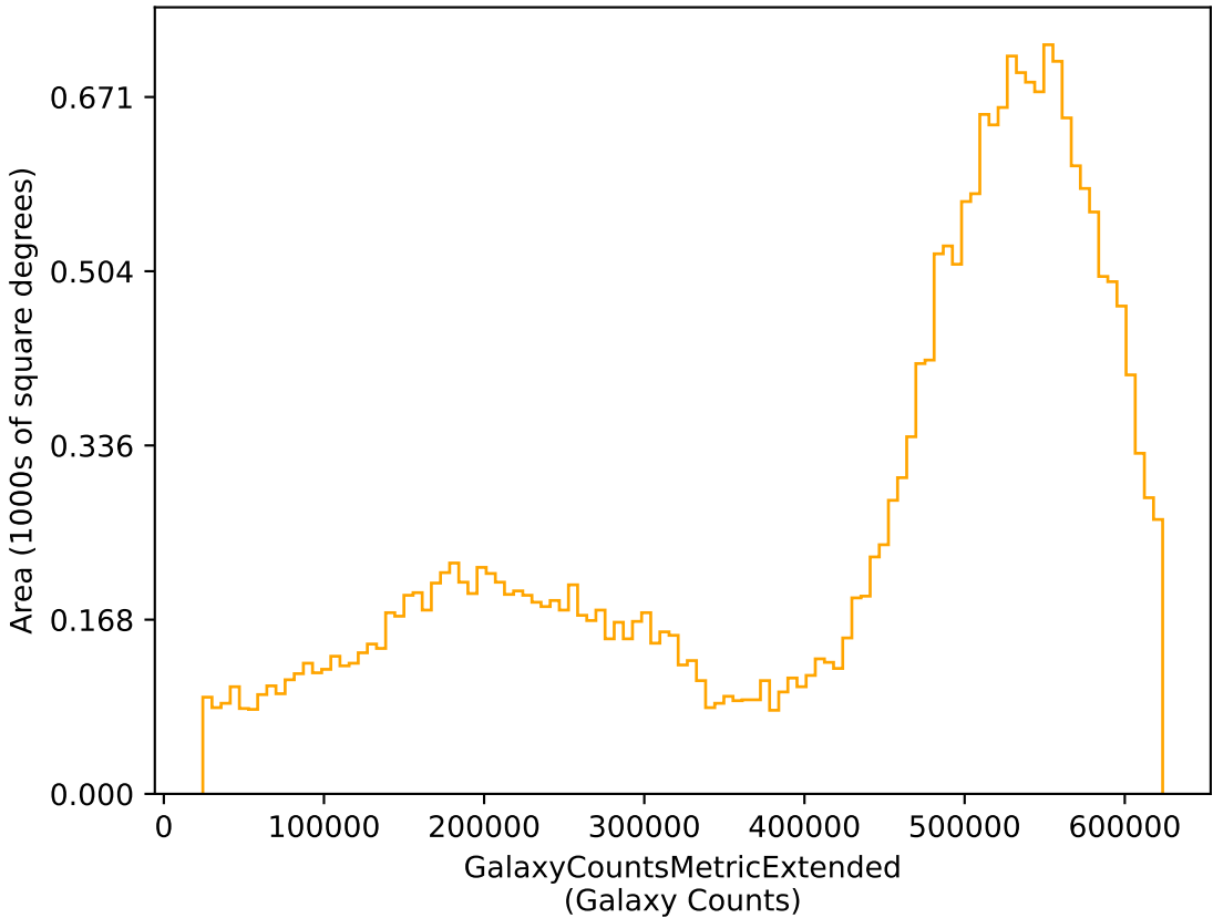
too_elab_r32_d2_giz_v3.4_10yrs r: GalaxyCountsMetricExtended
