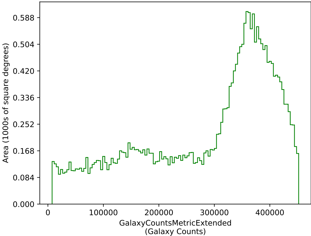
too_elab_r32_d2_giz_v3.4_10yrs g: GalaxyCountsMetricExtended
