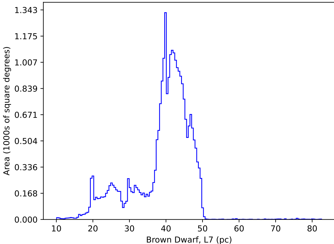
too_elab_r32_d2_giz_v3.4_10yrs : Brown Dwarf, L7
