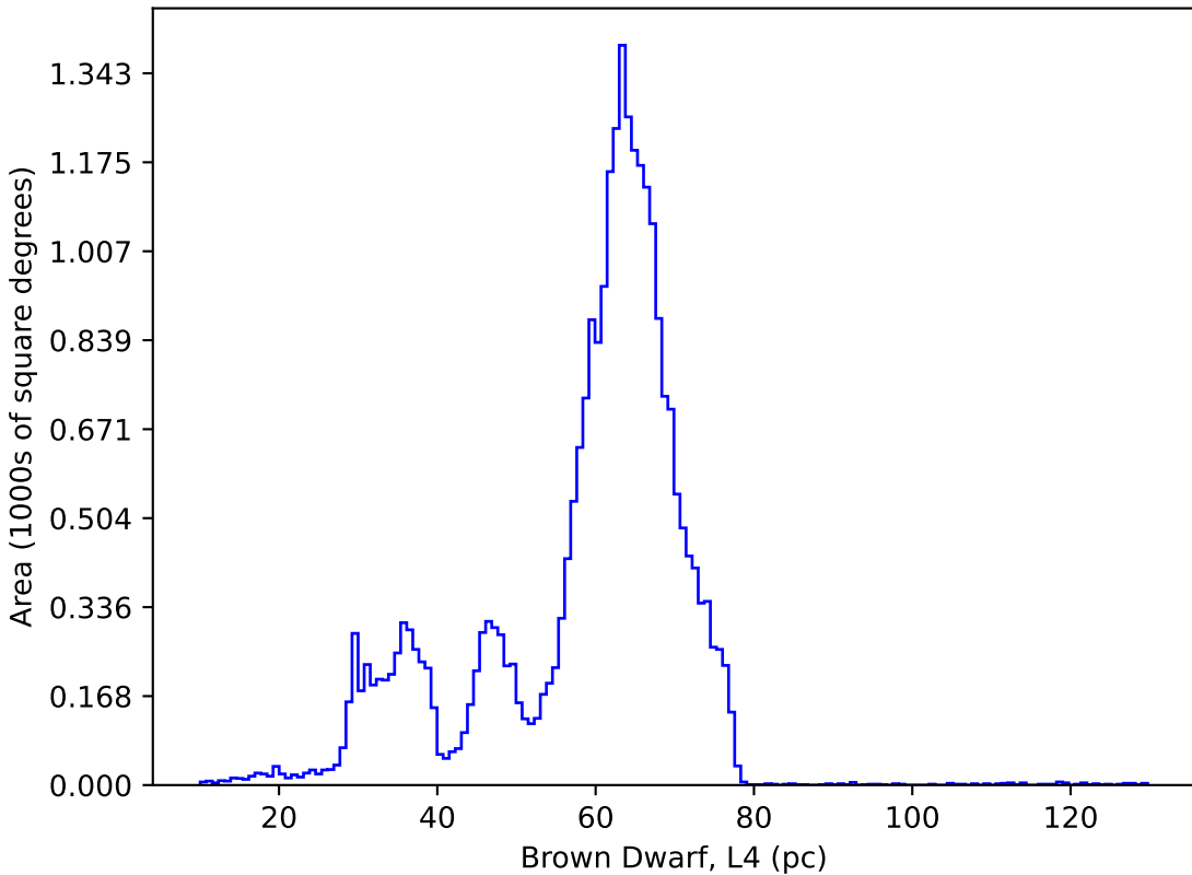
too_elab_r32_d2_giz_v3.4_10yrs : Brown Dwarf, L4
