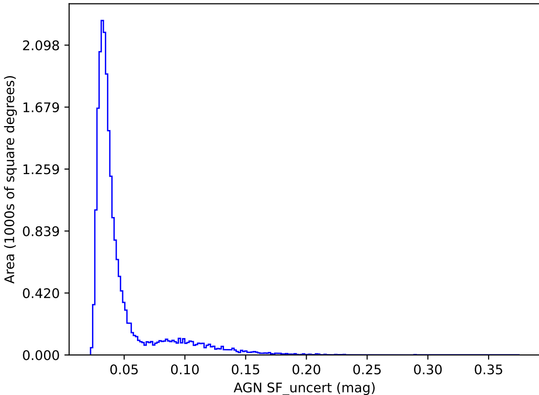
too_elab_r32_d2_giz_v3.4_10yrs y band: AGN SF_uncert
