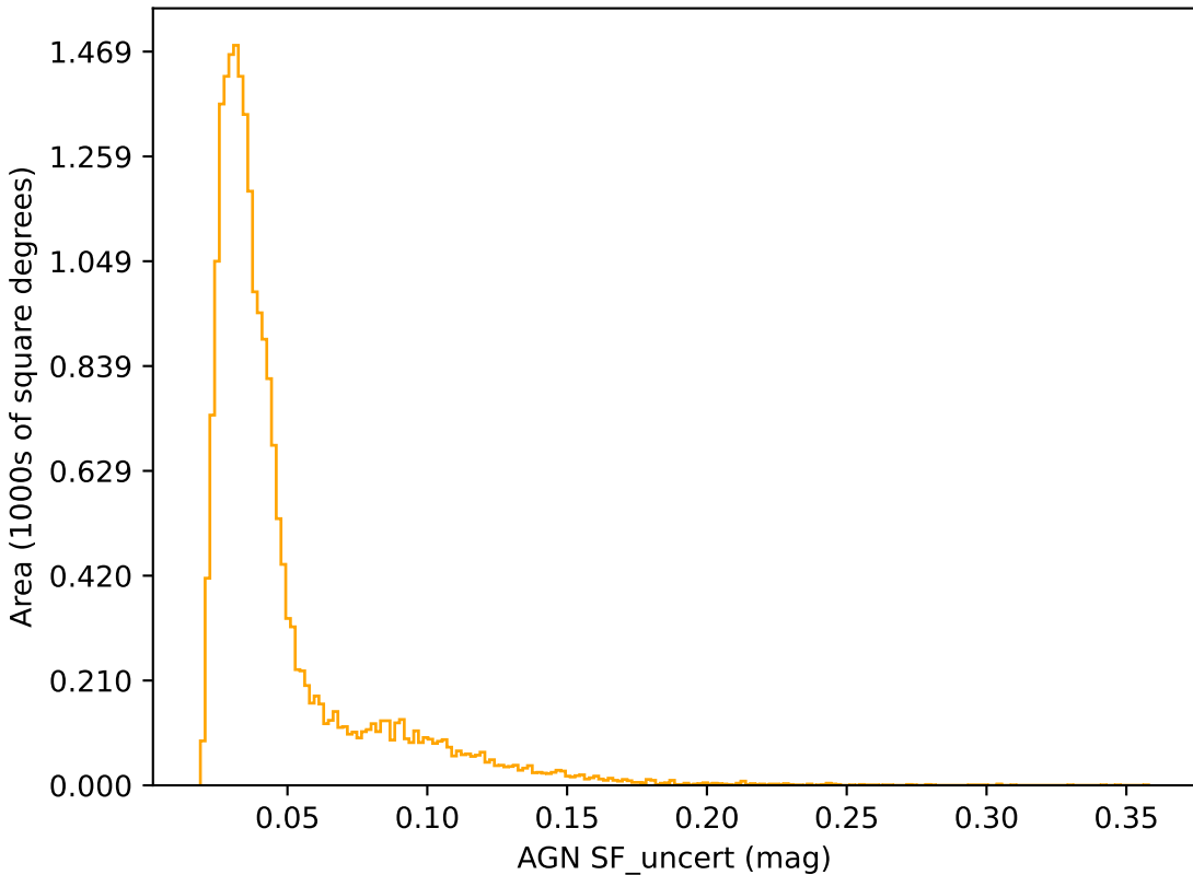
too_elab_r32_d2_giz_v3.4_10yrs r band: AGN SF_uncert
