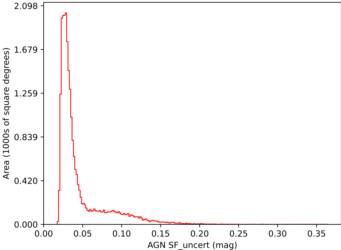
too_elab_r32_d2_giz_v3.4_10yrs i band: AGN SF_uncert
