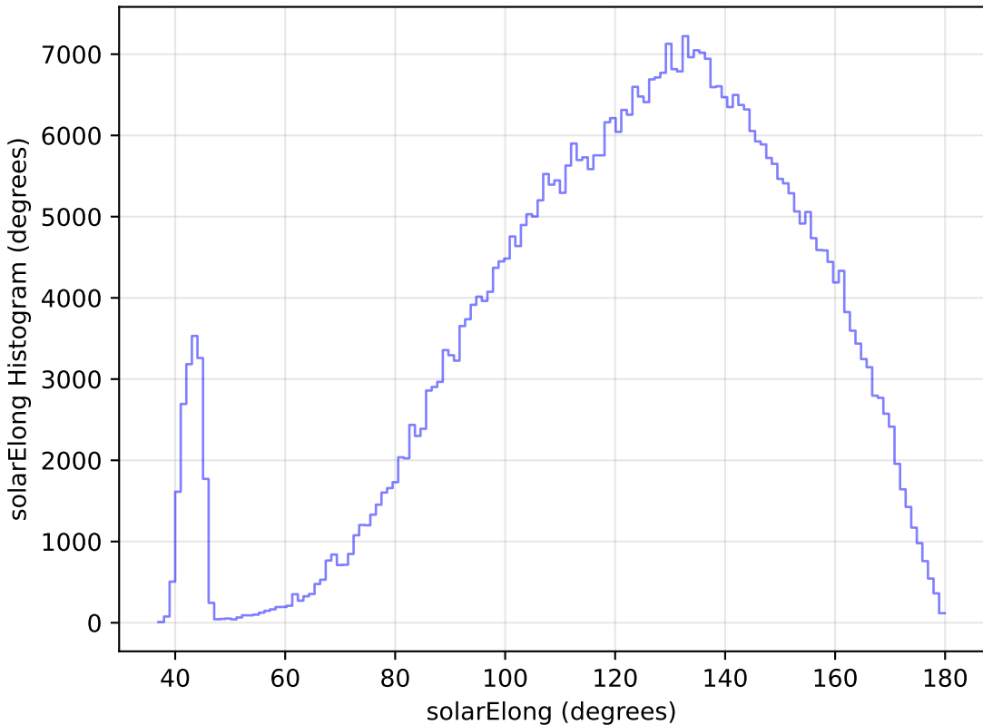
too_elab_r32_d2_giz_v3.4_10yrs WFD r band: solarElong Histogram
