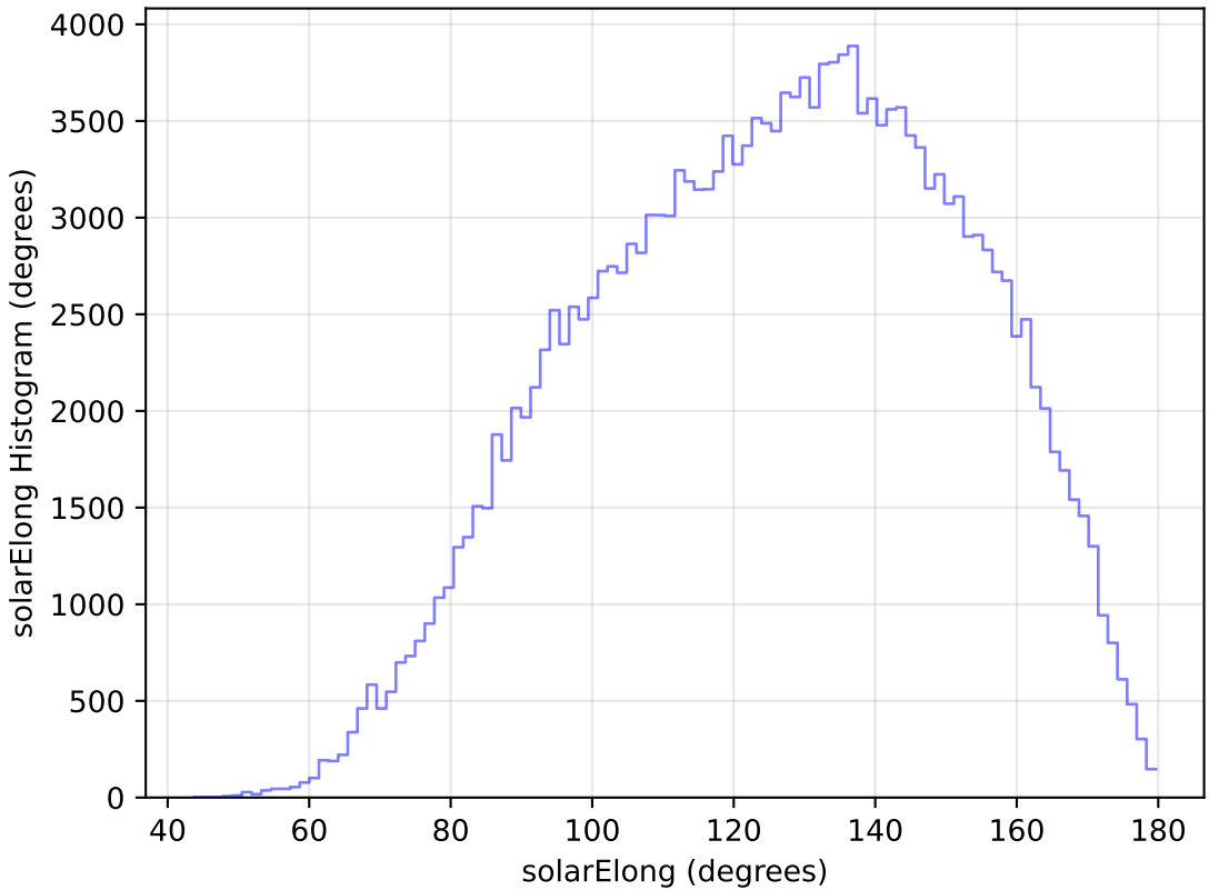
too_elab_r32_d2_giz_v3.4_10yrs WFD g band: solarElong Histogram
