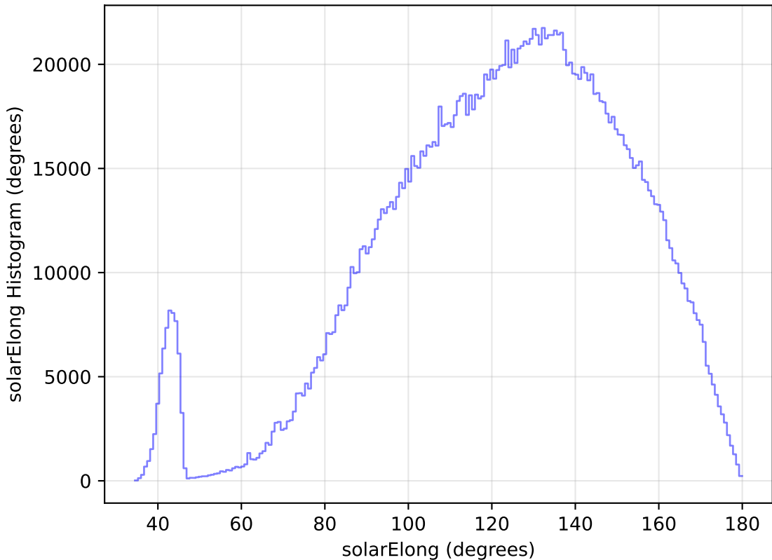
too_elab_r32_d2_giz_v3.4_10yrs WFD all bands: solarElong Histogram
