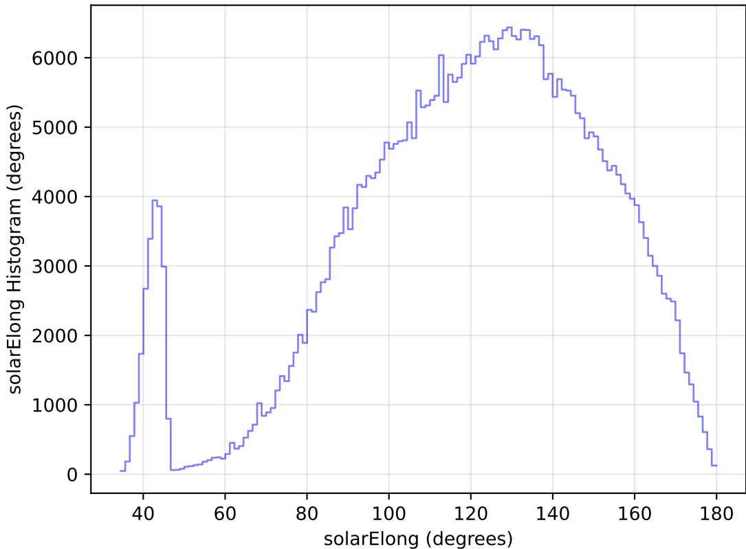
too_elab_r32_d2_giz_v3.4_10yrs All sky z band: solarElong Histogram
