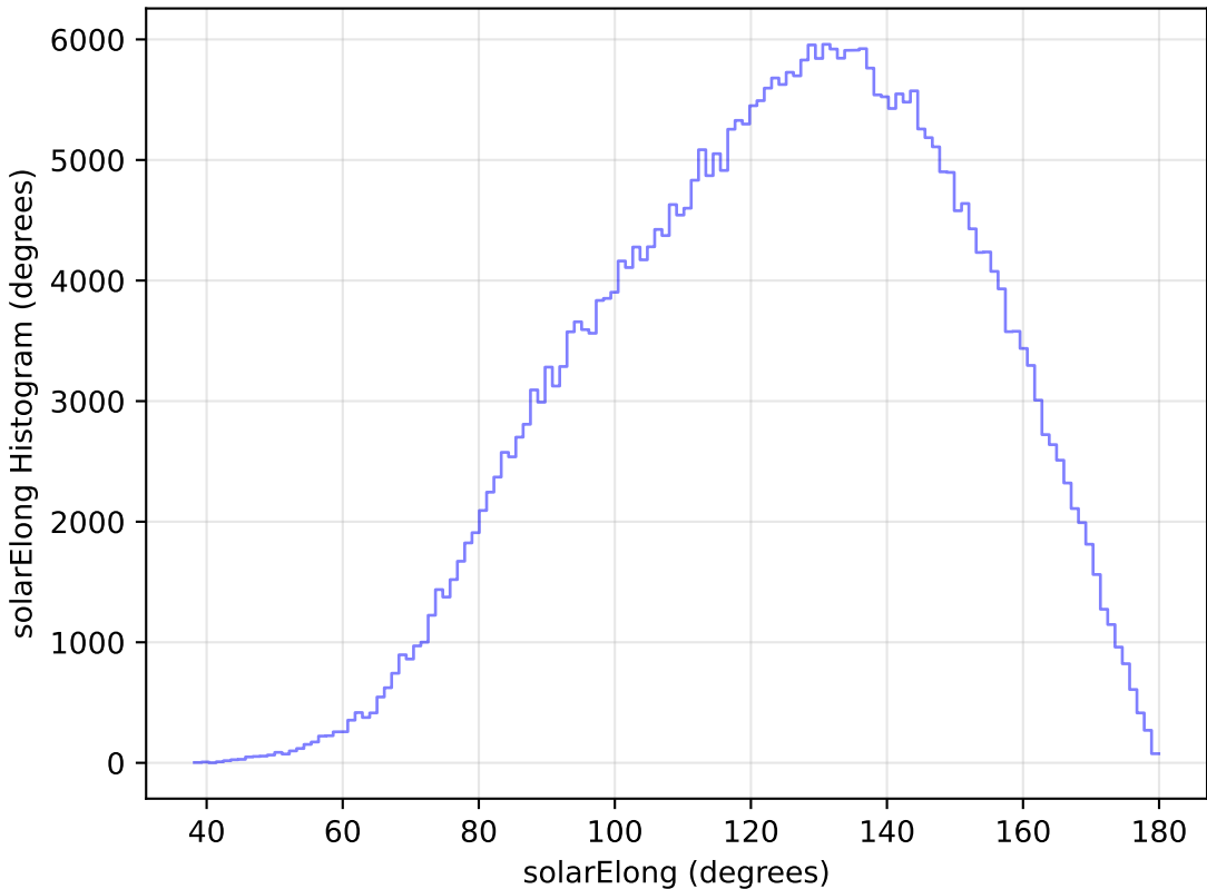
too_elab_r32_d2_giz_v3.4_10yrs All sky y band: solarElong Histogram
