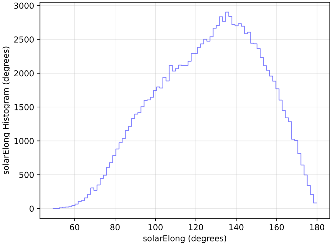
too_elab_r32_d2_giz_v3.4_10yrs All sky u band: solarElong Histogram
