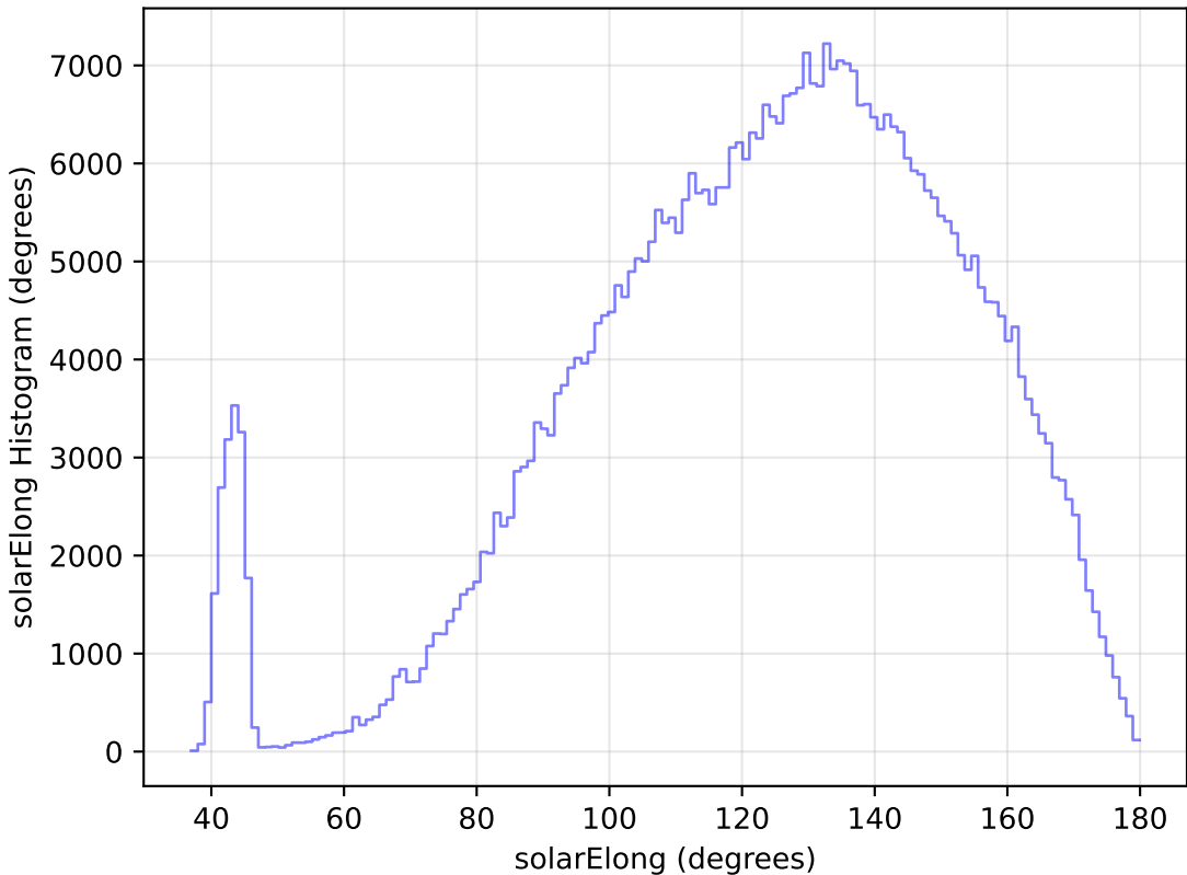
too_elab_r32_d2_giz_v3.4_10yrs All sky r band: solarElong Histogram
