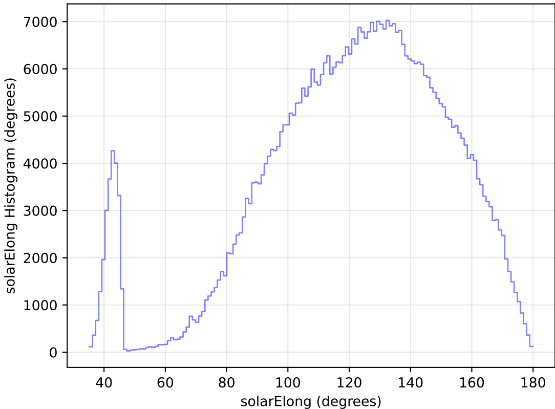
too_elab_r32_d2_giz_v3.4_10yrs All sky i band: solarElong Histogram
