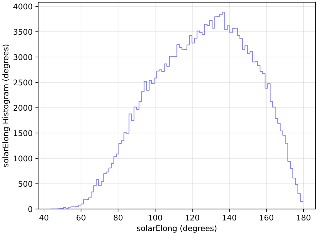
too_elab_r32_d2_giz_v3.4_10yrs All sky g band: solarElong Histogram
