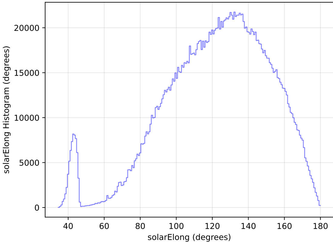
too_elab_r32_d2_giz_v3.4_10yrs All sky all bands: solarElong Histogram
