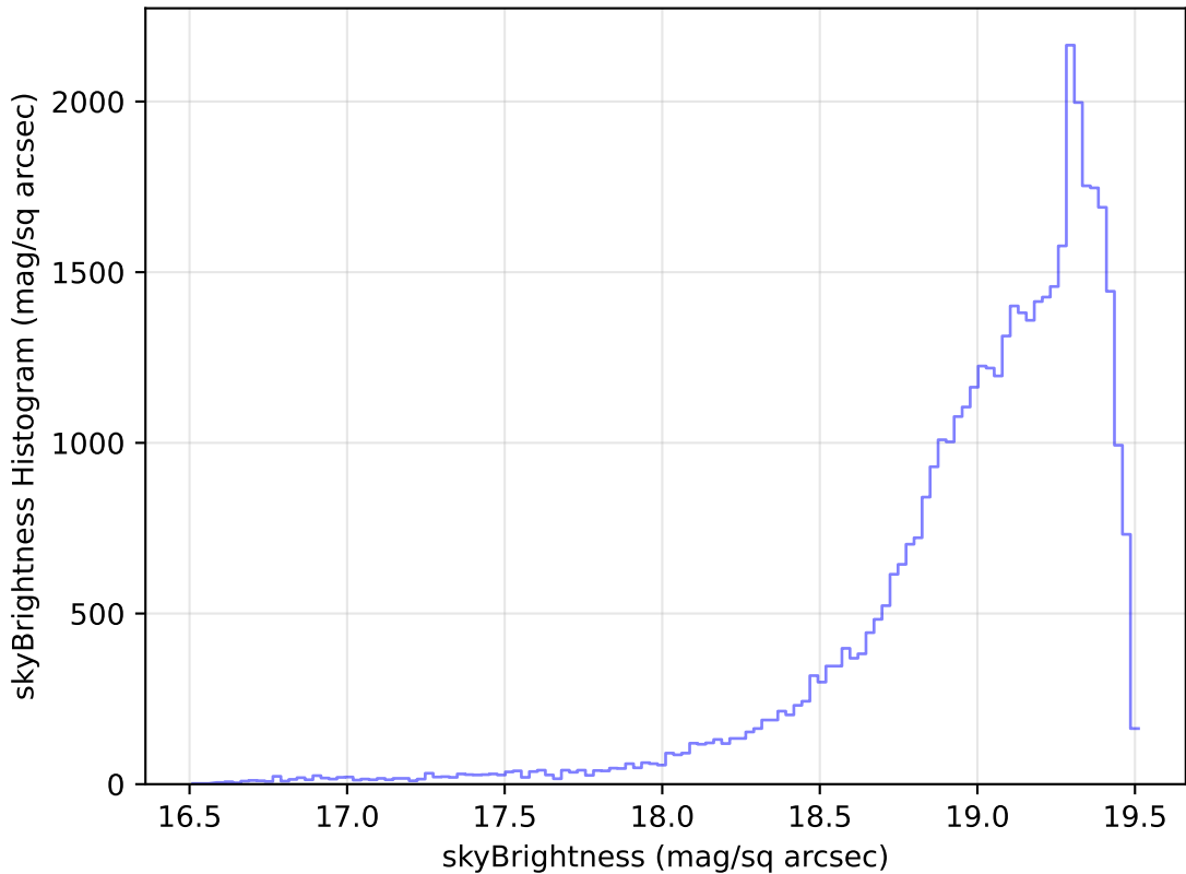
too_elab_r32_d2_giz_v3.4_10yrs Yr 1 z band: skyBrightness Histogram
