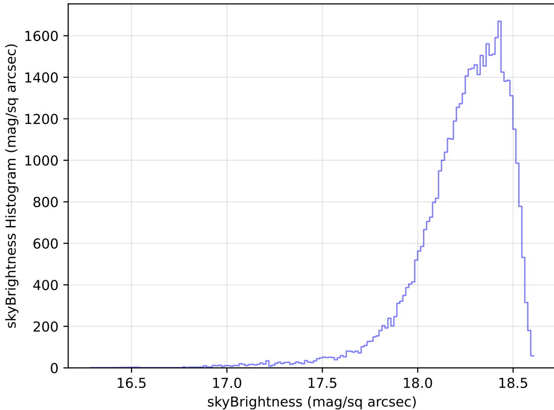
too_elab_r32_d2_giz_v3.4_10yrs Yr 1 y band: skyBrightness Histogram
