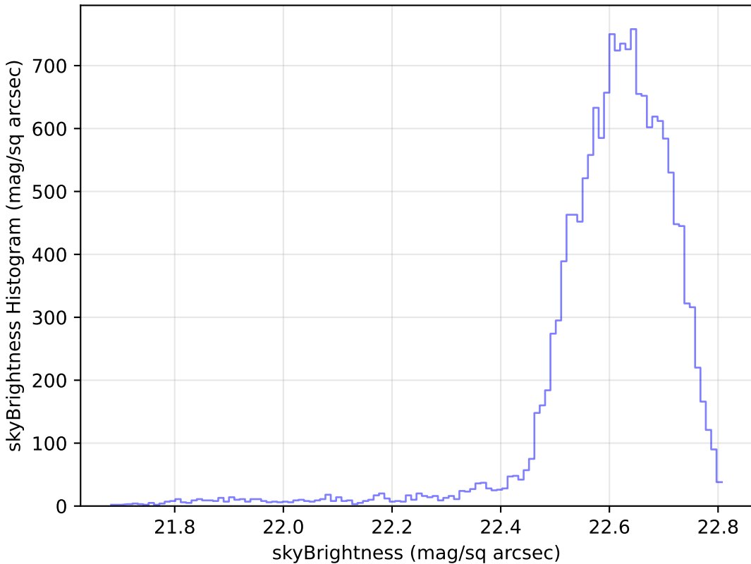
too_elab_r32_d2_giz_v3.4_10yrs Yr 1 u band: skyBrightness Histogram
