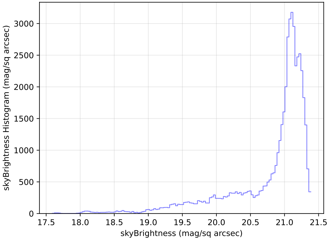
too_elab_r32_d2_giz_v3.4_10yrs Yr 1 r band: skyBrightness Histogram
