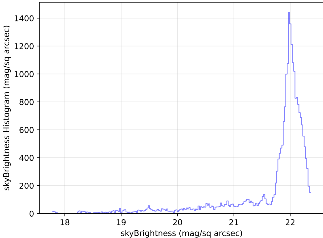
too_elab_r32_d2_giz_v3.4_10yrs Yr 1 g band: skyBrightness Histogram
