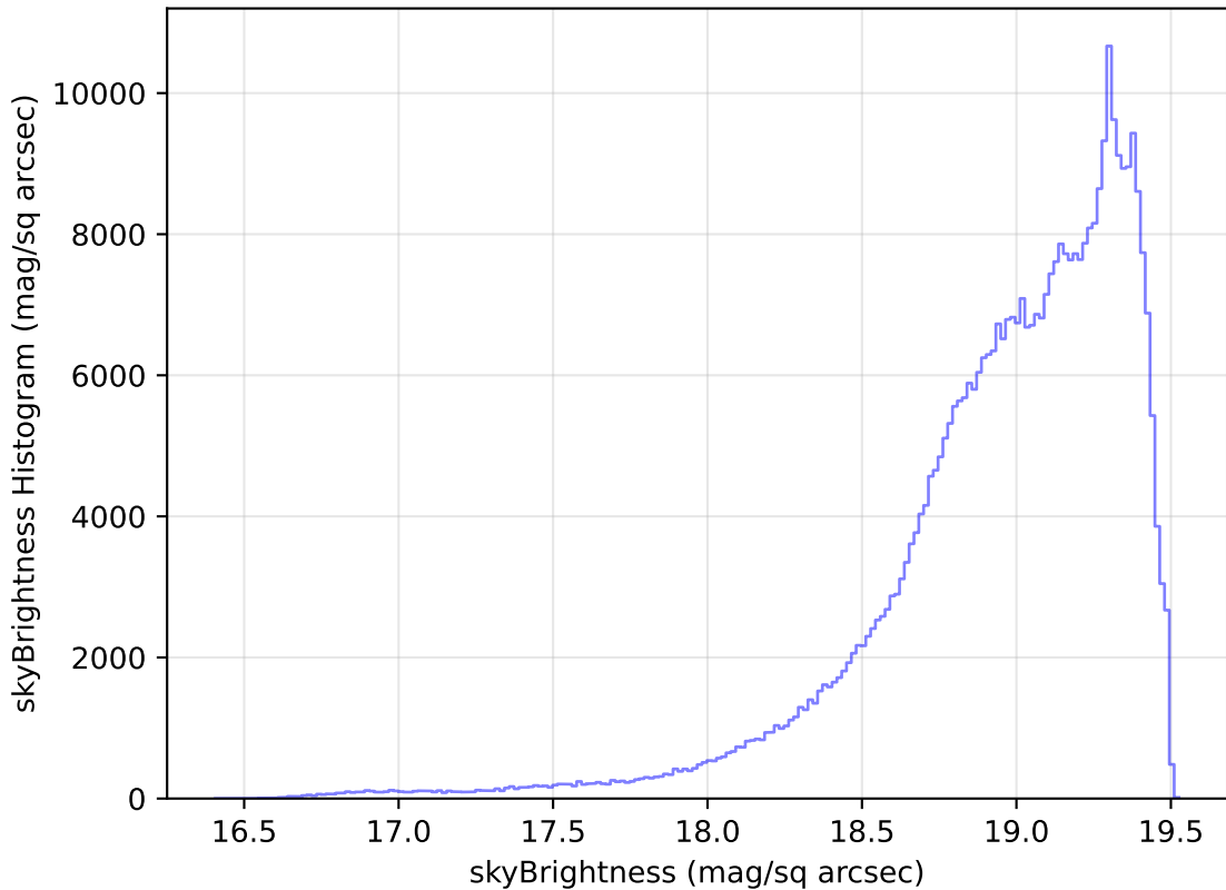
too_elab_r32_d2_giz_v3.4_10yrs WFD z band: skyBrightness Histogram
