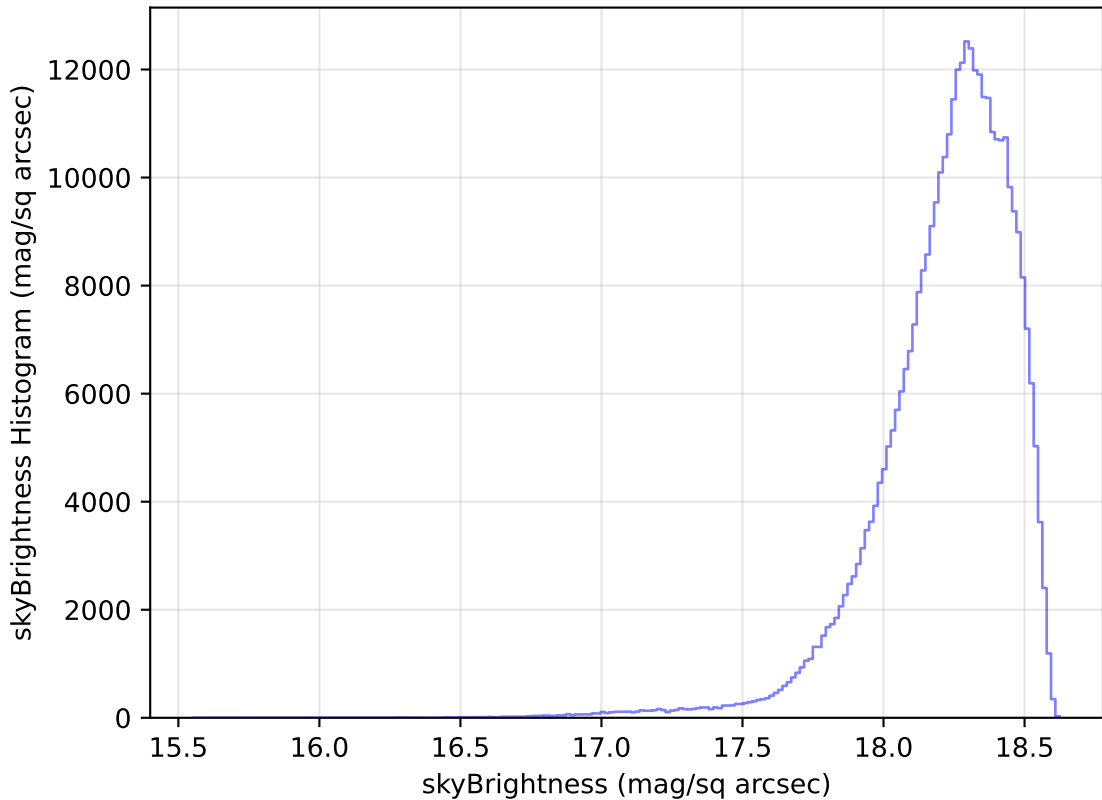
too_elab_r32_d2_giz_v3.4_10yrs WFD y band: skyBrightness Histogram
