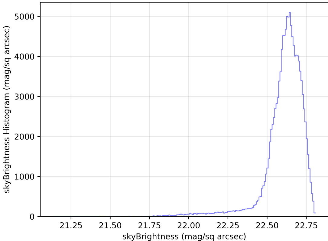
too_elab_r32_d2_giz_v3.4_10yrs WFD u band: skyBrightness Histogram
