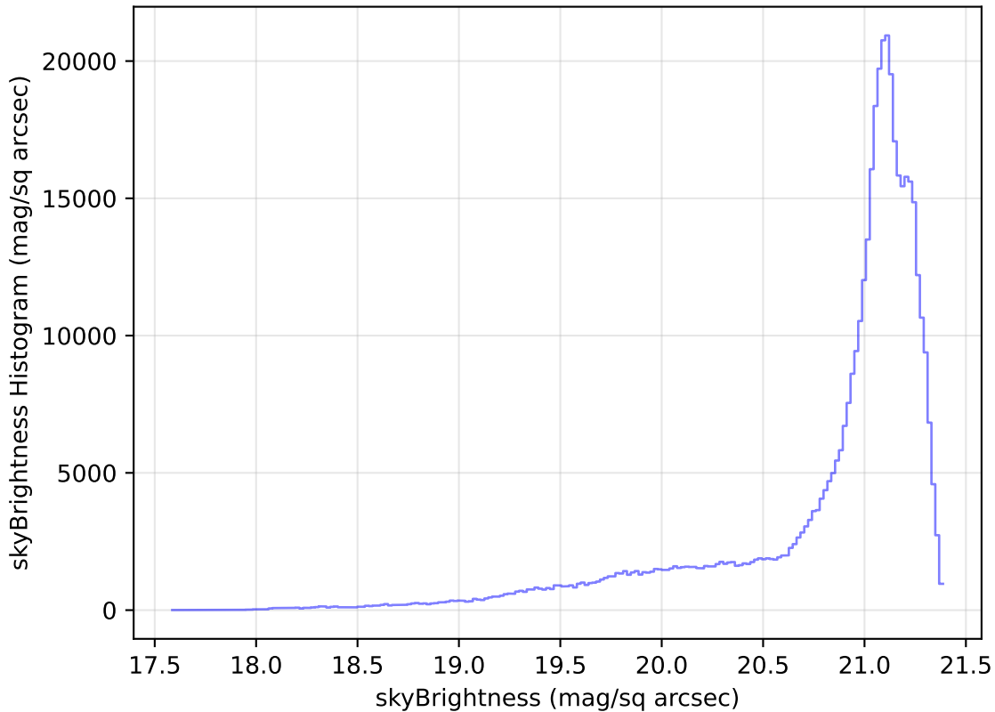
too_elab_r32_d2_giz_v3.4_10yrs WFD r band: skyBrightness Histogram
