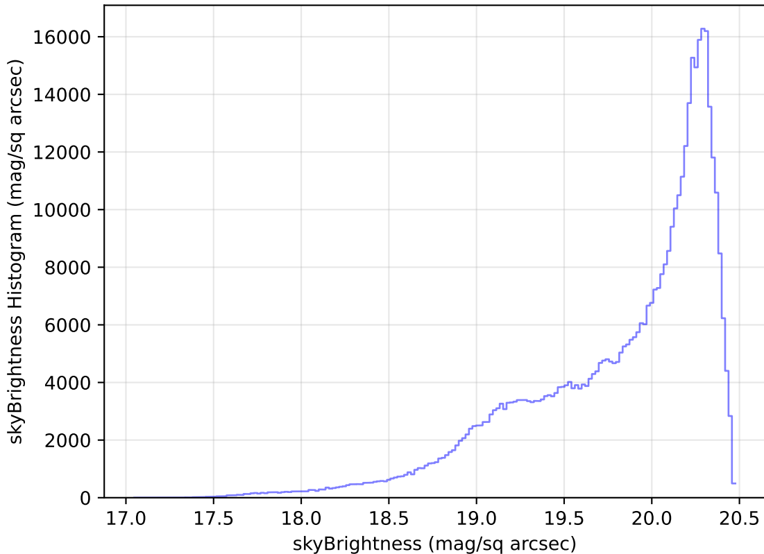
too_elab_r32_d2_giz_v3.4_10yrs WFD i band: skyBrightness Histogram
